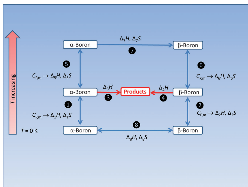
Figure 2. Thermodynamic cycle to determine relative stability of \alpha - and \beta -boron. The enthalpy difference between \alpha -boron and \beta -boron at T=0 K, \Delta_8 H , can be calculated if values for the other steps in a cycle (1, 3, 4, and 2, or 1, 5, 7, 6, and 2) are known.
